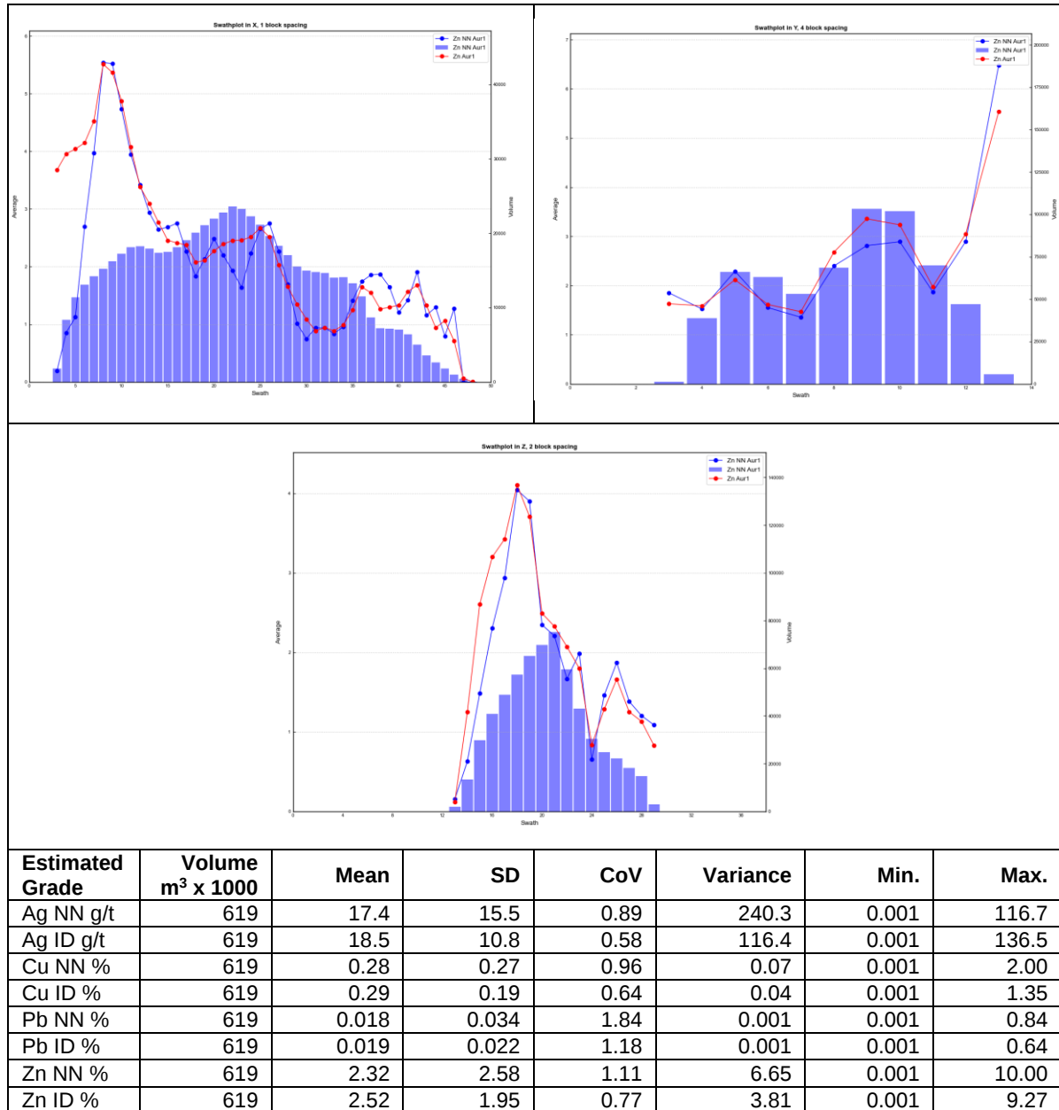
Figure 11-15 Zn Swath plots (X, Y and Z coordinate axes) and comparative statistics (Ag, Cu, Pb, Zn) – Aur-1 domain in Aurora
