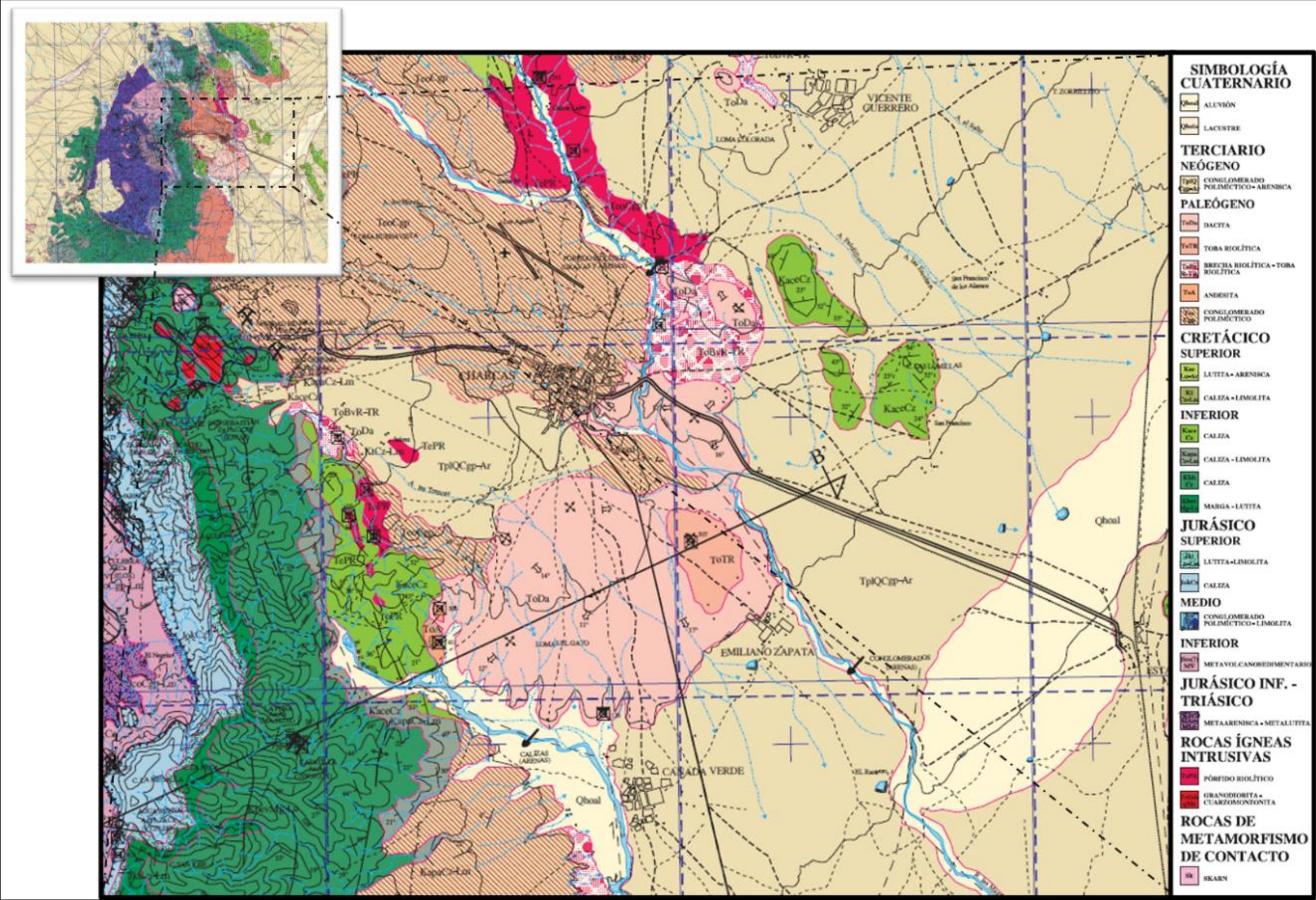
Figure 6-1Regional Geology Map
