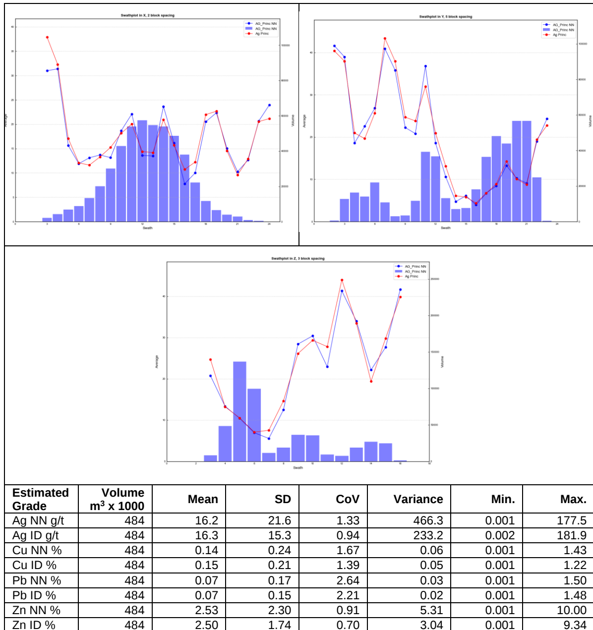
Figure 11-14 Ag Swath plots (X, Y and Z coordinate axes) and comparative statistics (Ag, Cu, Pb, Zn) – Principal domain in Las Eulalias
