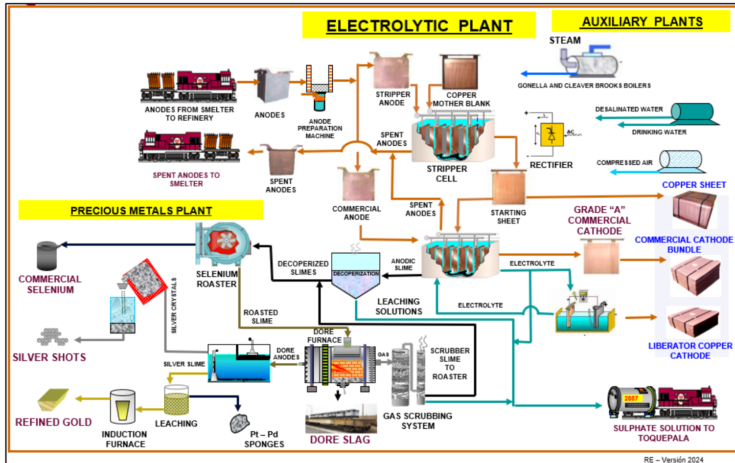
Figure 14-5: Summary Flowsheet Ilo Refinery
