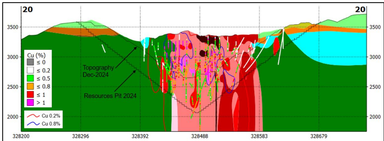
Figure 6-6: Geological Cross-section 20
