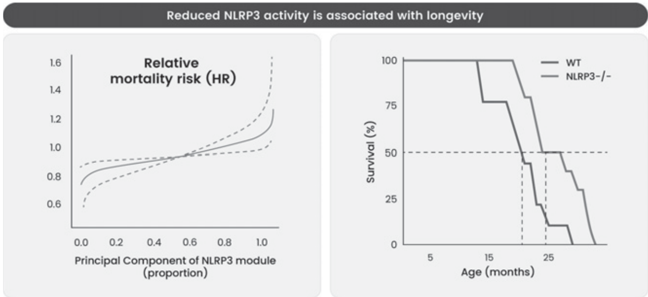
Levels of NLRP3-associated proteins (principal component) are inversely related to mortality risk in our human aging cohorts (left). Consistently, in a third-party preclinical study, knockout of the NLRP3 gene in mice significantly extends lifespan ( n = 10 mice per group) (right). (Source: Marín-Aguilar et al. 2020).
